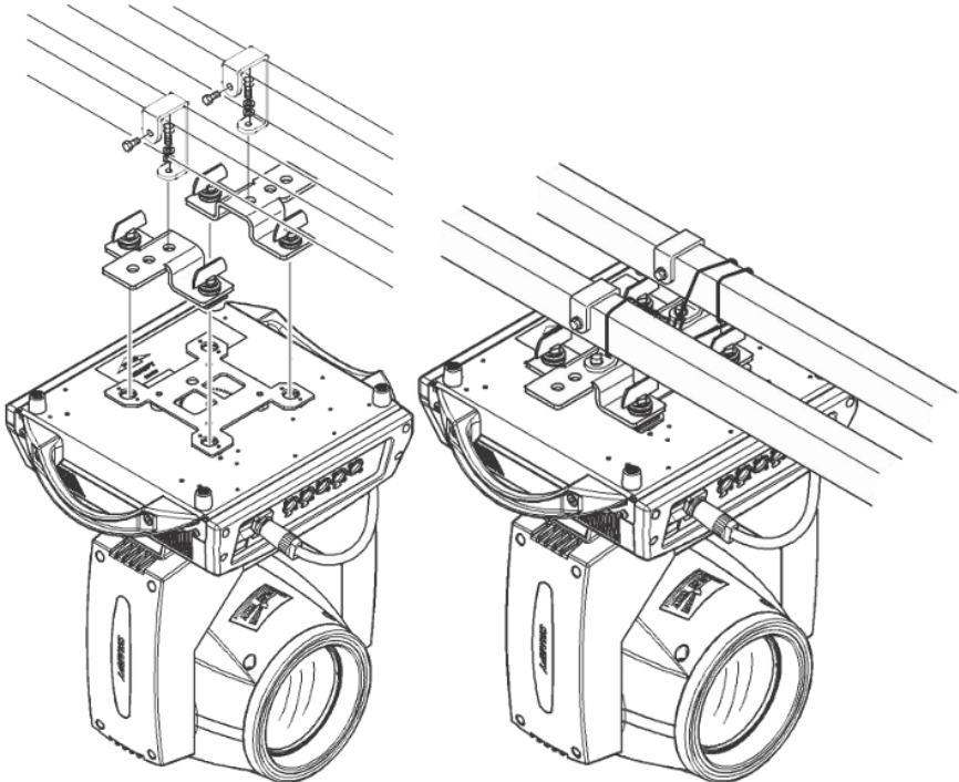
Figure 2 Diagram of the Installation
